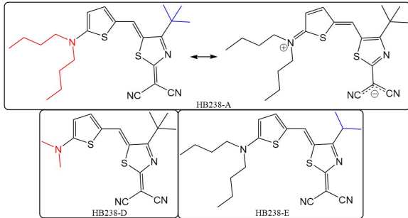
Structures of studied molecules
