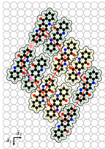
\beta -phase of Quinacridone on Ag(100).
