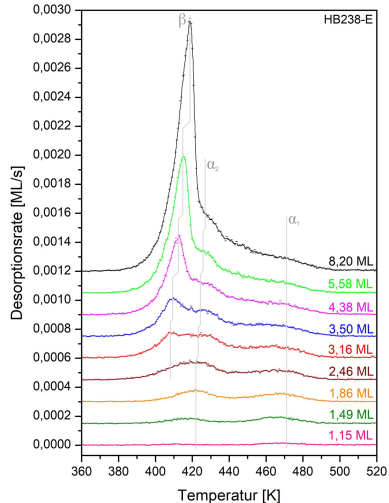
TPD spectra of HB238-E on Ag(100)
