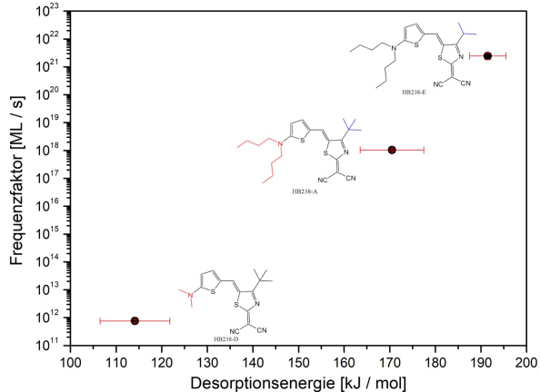
Desorption energy vs. pre-exponential factor
