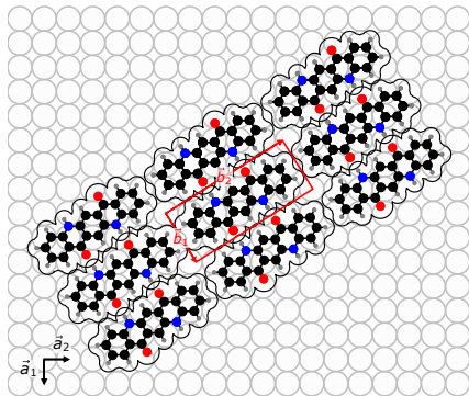
\alpha -phase of Quinacridone on Ag(100).
