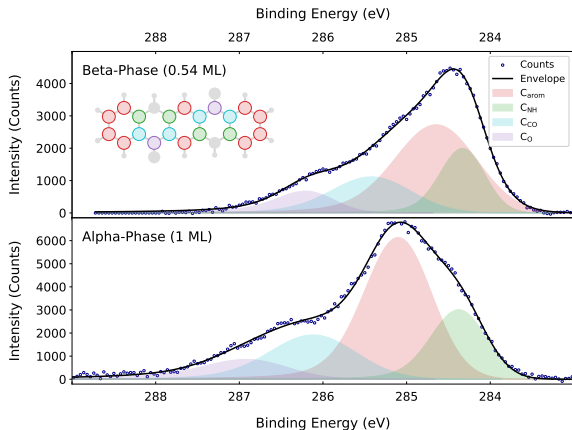
C1s XPS spectra of Quinacridone on Ag(100)
